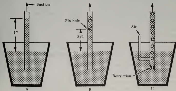
FIGURE 3-9. Air bleed principle.
